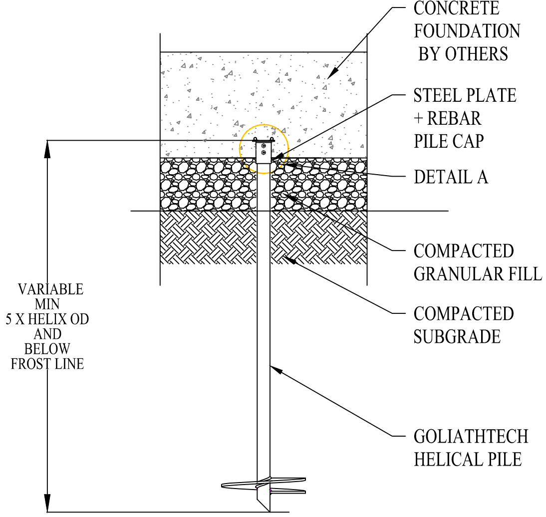
SIDE VIEW
